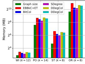
Figure 11: Space costs.
