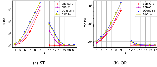
Figure 14: Ablation studies.
